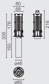
POWER LED 10W
