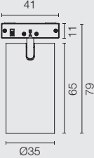
LIGHT STRIPE WALL-WASHER
