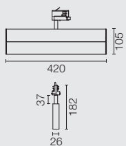
TOP LED 25,5W
