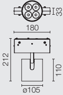
POWER LED 13W
