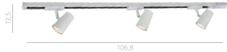
914003 GU10 3x35W
