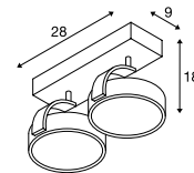
Dimensional drawing
